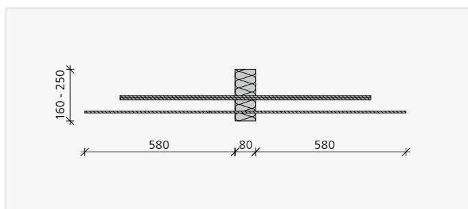
ISOPRO® IPE 1
