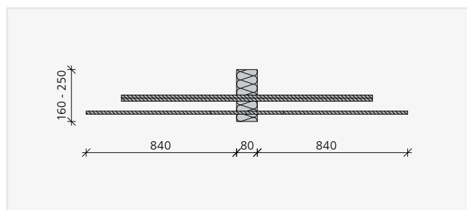
ISOPRO® IPE 2
